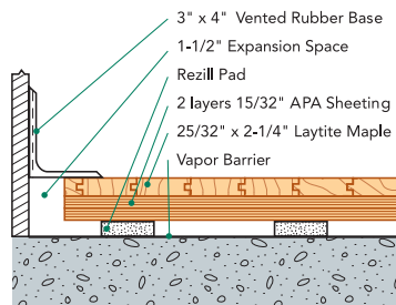
THRESHOLD DETAIL (optional accessory)
