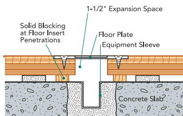
EQUIPMENT DETAIL (optional accessory)
